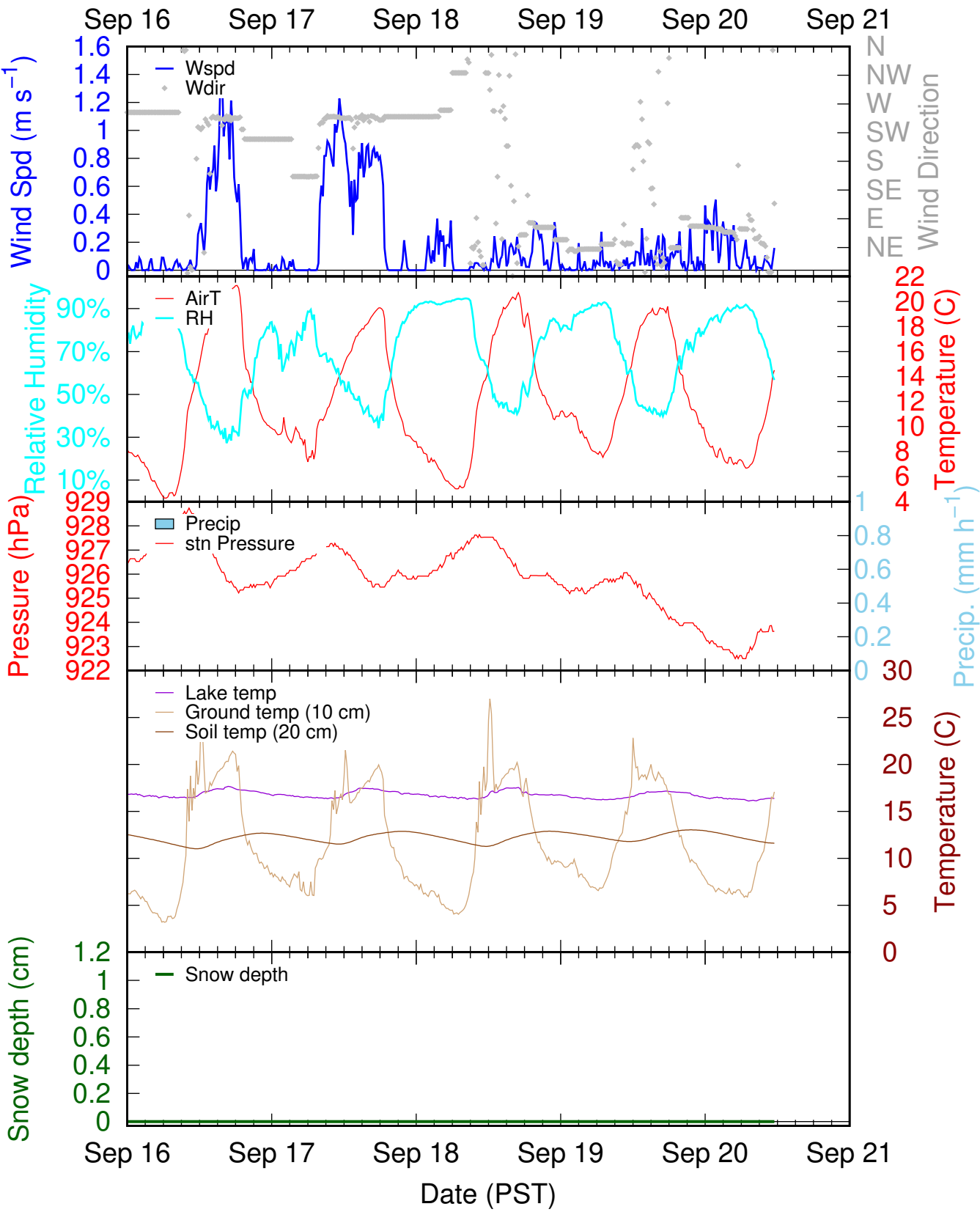
Ness Lake weather station (15 min avg) on Sun Sep 20 11:33:02 PDT 2026
